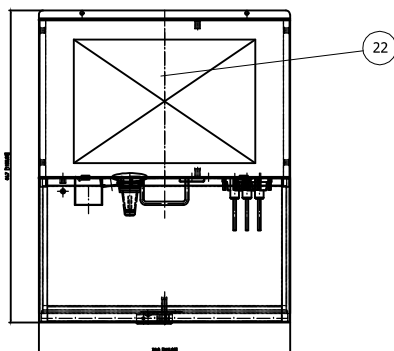
L.V. TERMINAL DETAIL
